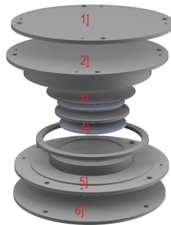
Fixed Spherical Bearing
